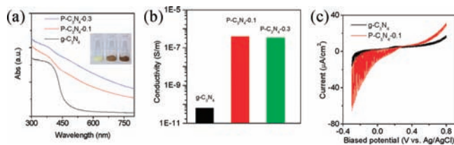
Figure 2. UV-vis spectra (a) and electrical conductivity (b) of P doped and pristine g\text{-C}_3\text{N}_4 . Inset: photographs for g\text{-C}_3\text{N}_4 (left), \text{P-C}_3\text{N}_4\text{-0.1} (middle), and \text{P-C}_3\text{N}_4\text{-0.3} (right). (c) Current-potential curve of P-doped and pristine g\text{-C}_3\text{N}_4 photoelectrodes in 0.1 M aqueous KCl under chopped visible light ( \lambda > 420 nm, 150 W Xe lamp), chopping frequency: \sim 0.5 Hz, scan rate: 10 mV/s.
