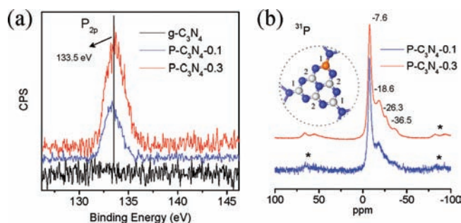
Figure 1. (a) XPS and (b) 31 P solid-state MAS NMR spectra of P-doped and pristine g-C 3 N 4 . The asterisks mark spinning sidebands. Inset: the building unit of C 3 N 4 with P doping at the corner-carbon site (1, the substitution at bay-carbon site, 2, is not shown). Carbon atoms are gray, nitrogen atoms are blue, and phosphorus atom is orange.
